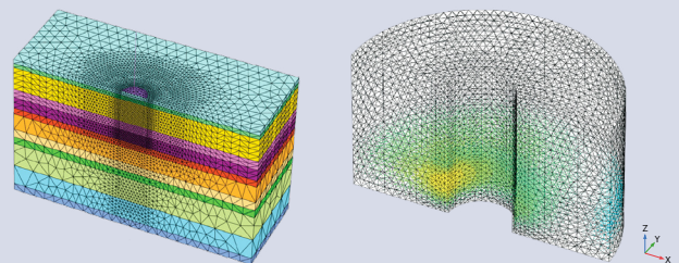
Detailed 3-D FE-Analysis of the pore water pressure development adjacent to a Monopile in a maximum storm event.
